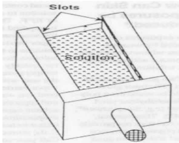
Figure 3 – Slot Hood for Dip Tank
